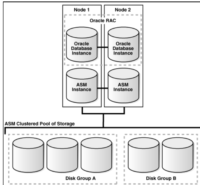
Figure 1–2 Oracle Instances and Oracle ASM Storage
