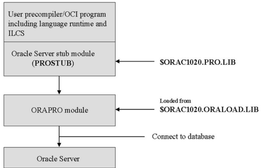
Figure 5–1 Usage of Program Libraries by Programmatic Interfaces
